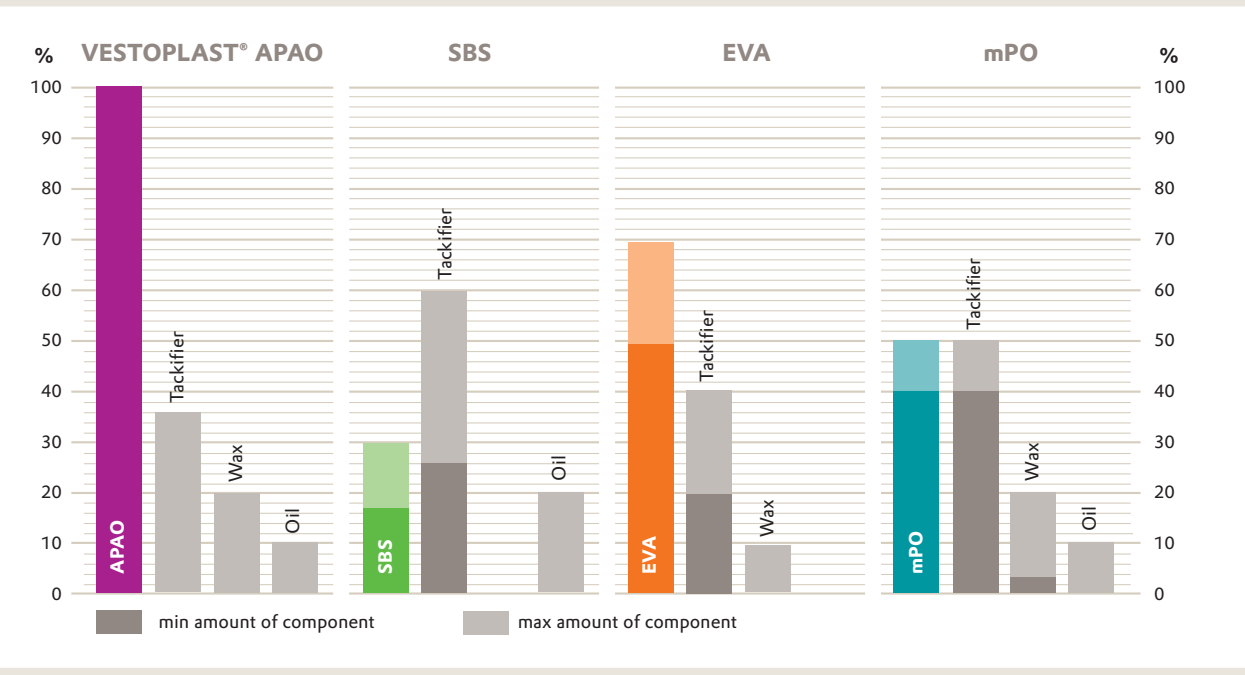
Formulation window of various polymers and additives
